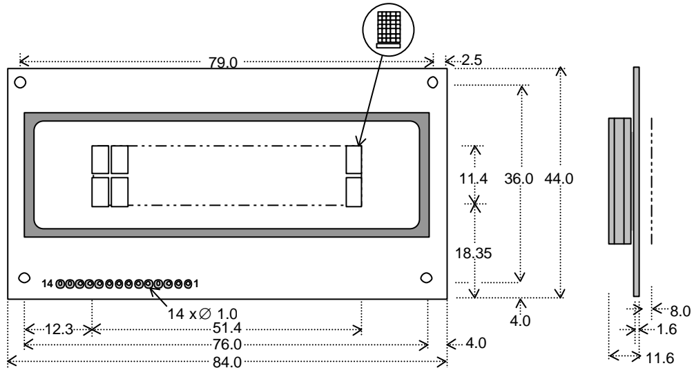
Dimensions in mm & subject to tolerances. Mounting holes 2.8mm dia.
