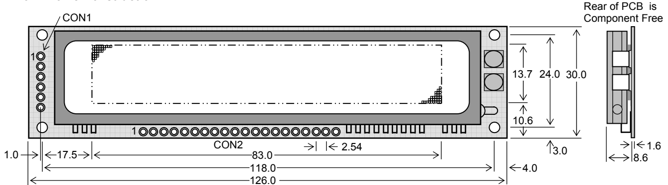
Dimensions in mm & subject to tolerances. Mounting holes 3.5mm dia.
