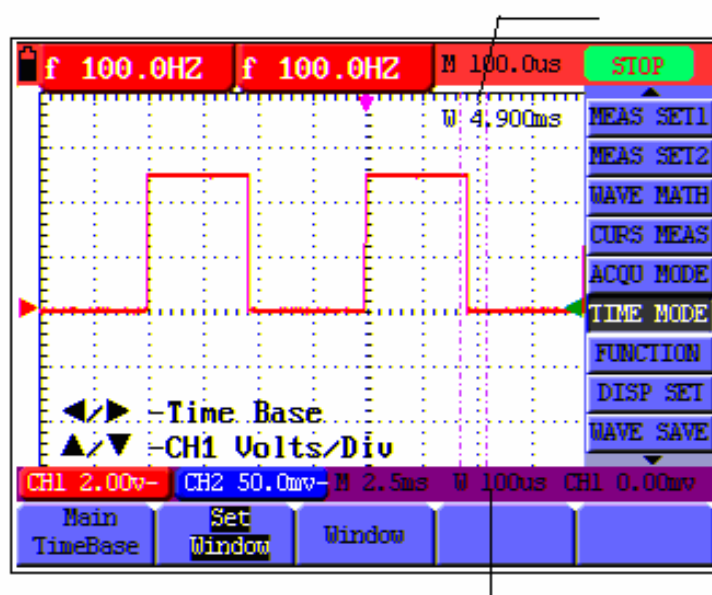
figure 57: Window Setting
