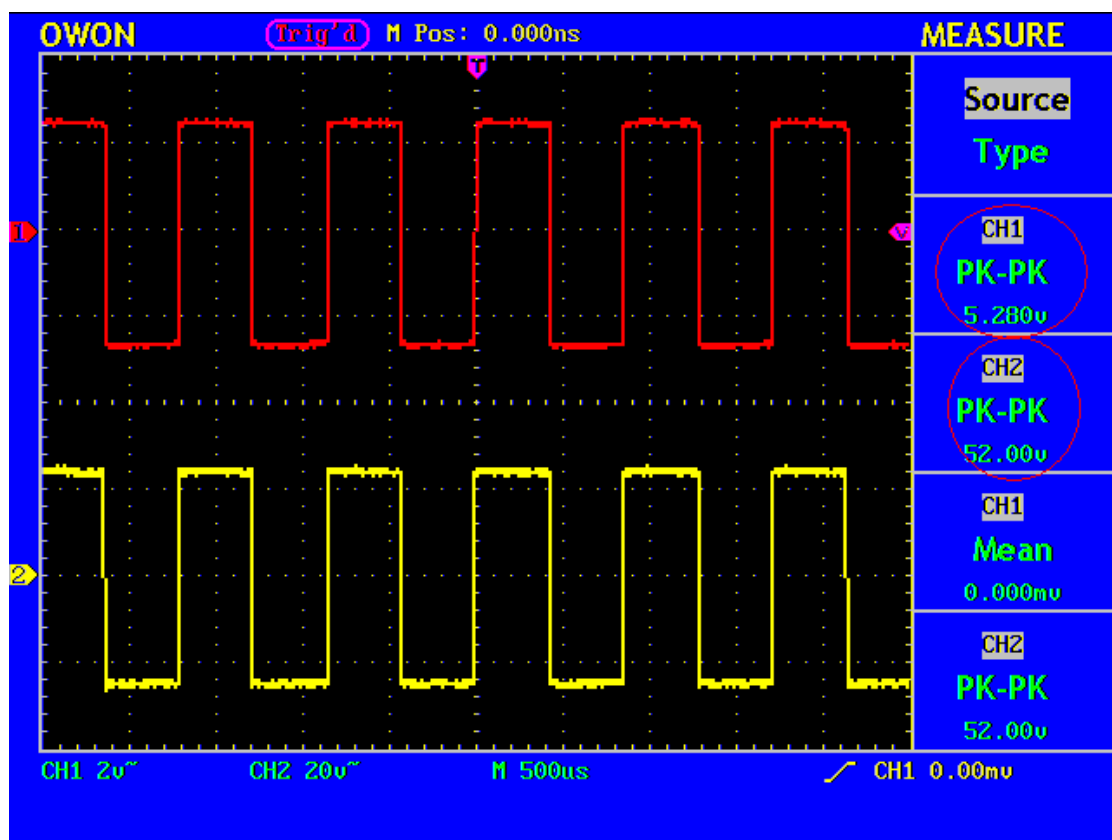
Fig. 56 Wave Form of Gain Measurement
