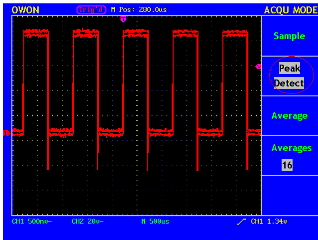
Fig. 37 Peak Detect mode, under which the burrs on the falling edge of the square wave, can be detected and the noise is heavy.
