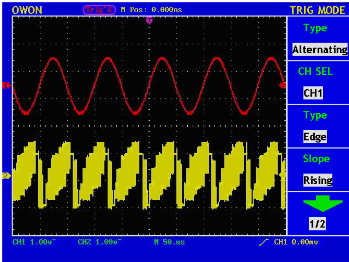
Fig 35 Alterate trigger waveform
