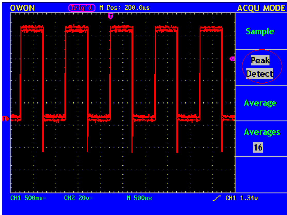
Fig. 58 Wave Form of the Signal Containing Noises
