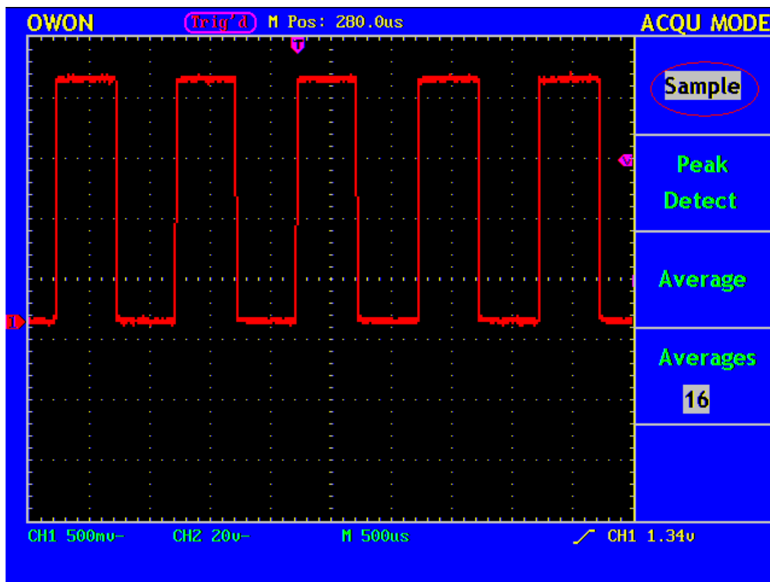
Fig. 38 Common ACQU Mode display, in which no burr can be detected.
