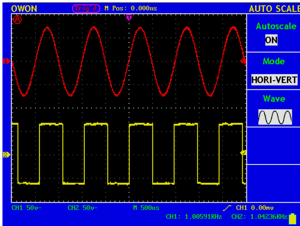
Fig1: Autoscale Horizontal- Vertical multi-period waveforms
