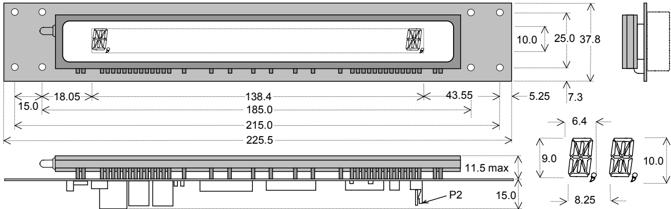
Dimensions in mm & subject to tolerances. Mounting holes 4.0mm dia.
